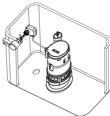
Flush Valve Assembly with Flush Lever (Color Match) PF9812FVPK
