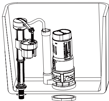
Fill Valve Assembly PF9812FLPK
